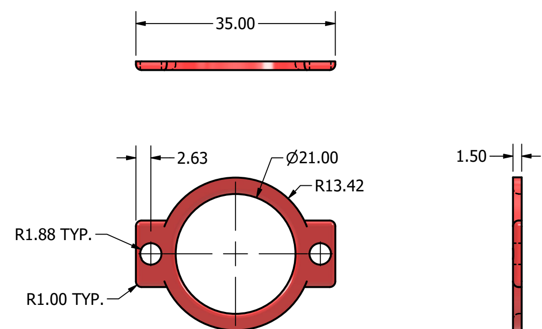
FLASHLIGHT PLATE SCALE 1.5:1
