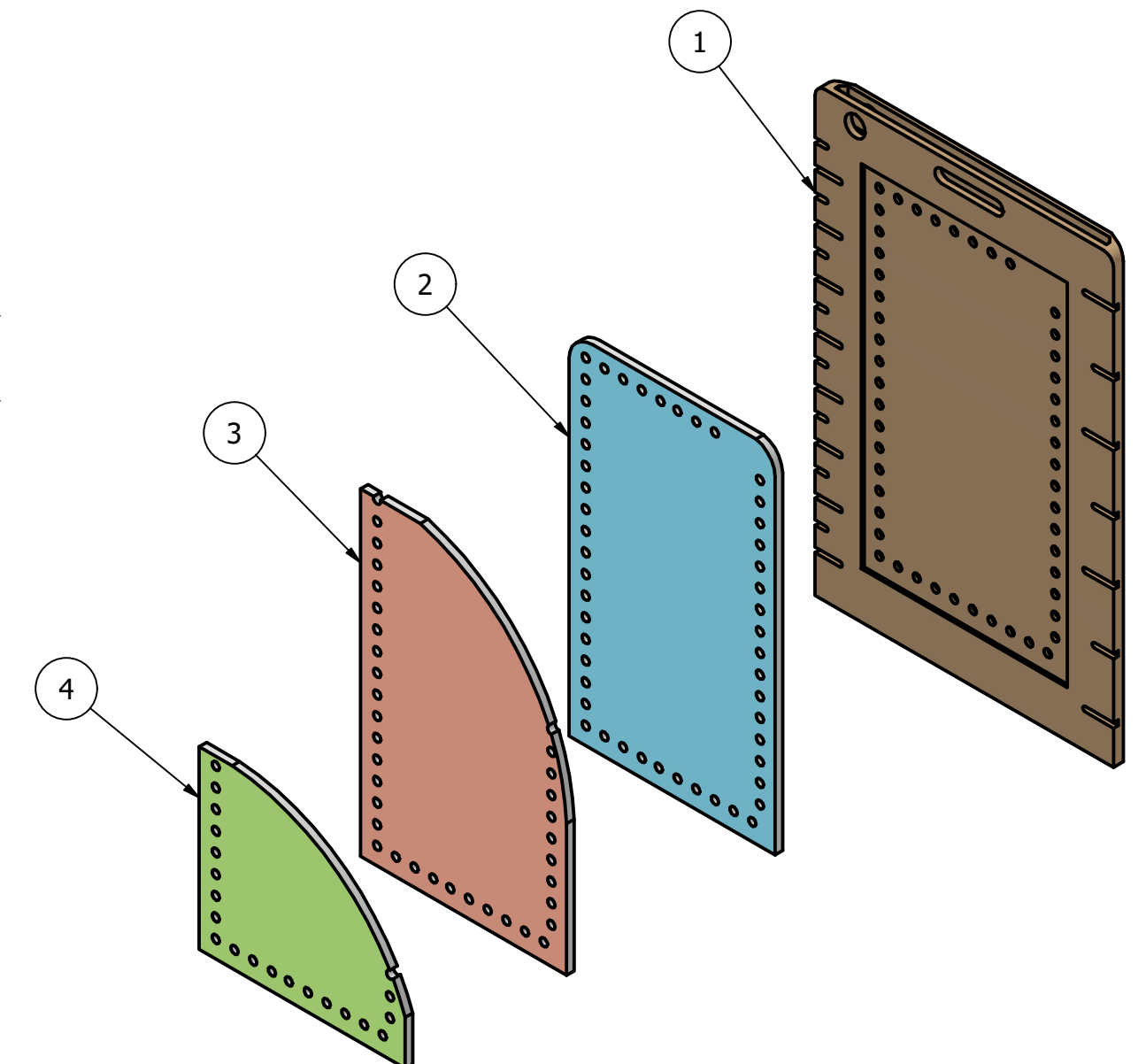
EXPLODED VIEW SCALE 1:1
