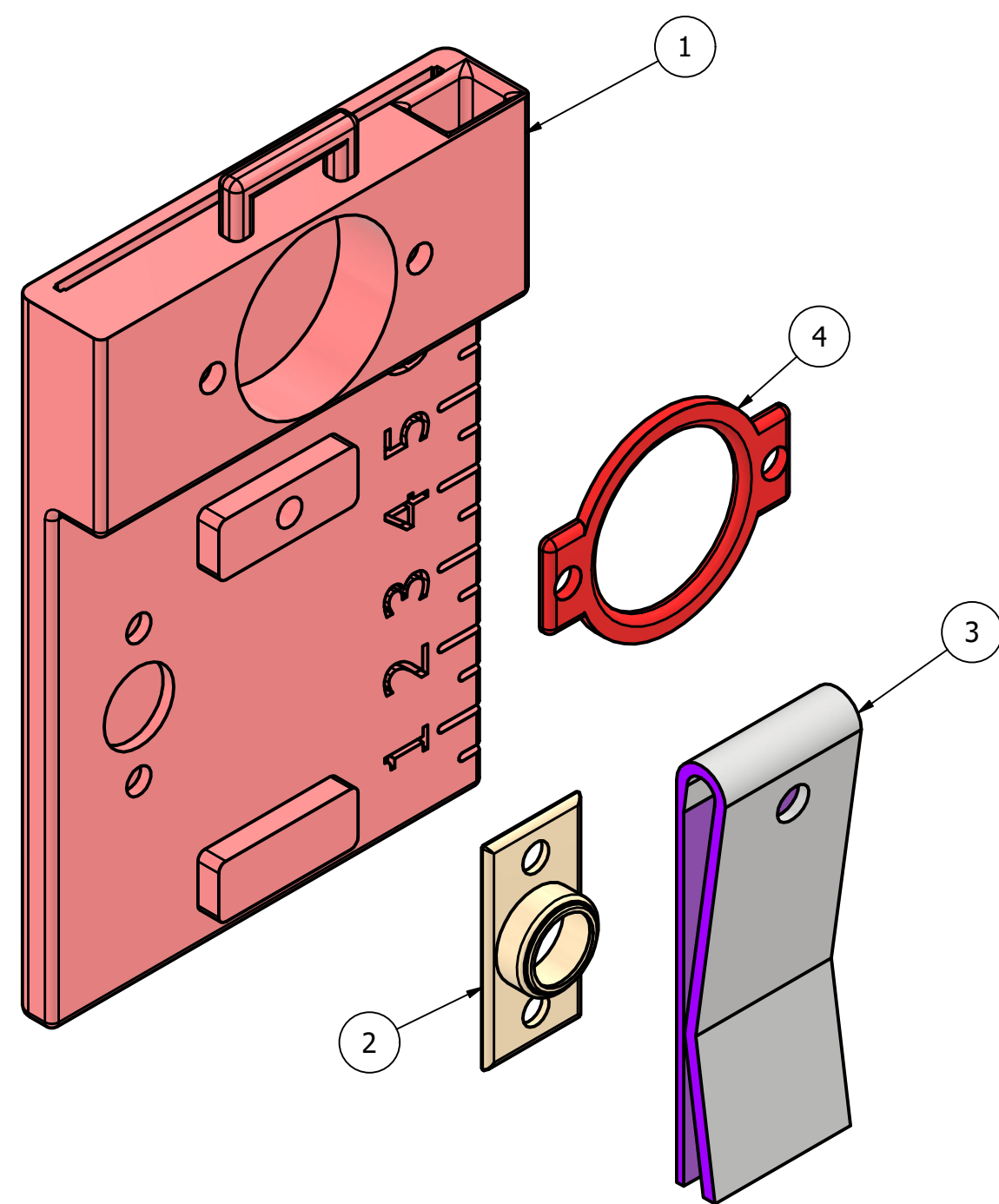
EXPLODED VIEW SCALE 1.5:1
