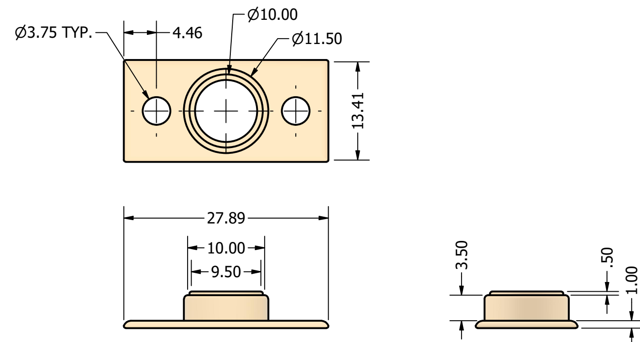
LEVELER PLATE SCALE 2:1
